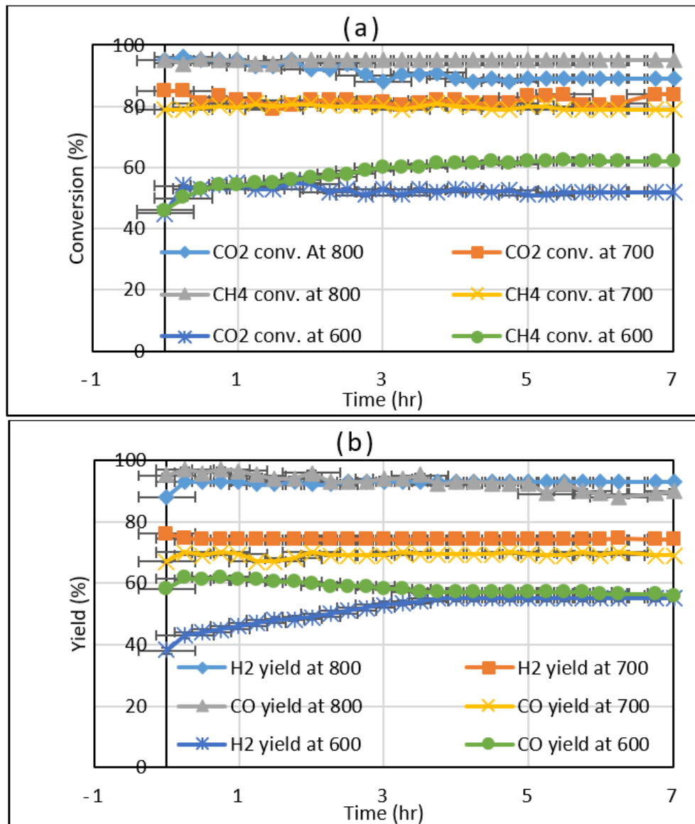
Fig. 6 Catalytic Results: (a) CH 4 and CO 2 Conversion (b) H 2 /CO Yield [121].
