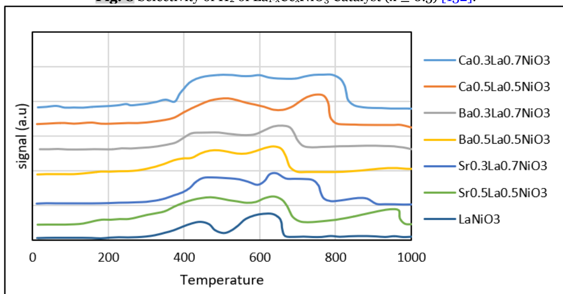
Fig. 9 \text{H}_2 -TPR Profiles of \text{M}(\text{Ca, Ba, Sr})_x\text{La}_{1-x}\text{NiO}_3 ( x = 0.0, 0.3, 0.5 ) Perovskites [117].
