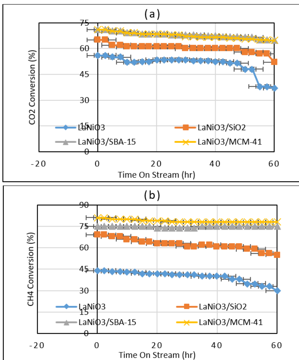
Fig. 16 Catalytic Stability of Bulk and Supported \text{LaNiO}_3 Catalysts for the CDRM Reaction at 700 °C for 60 h, (a) \text{CO}_2 Conversion%, (b) \text{CH}_4 Conversion% [83].
