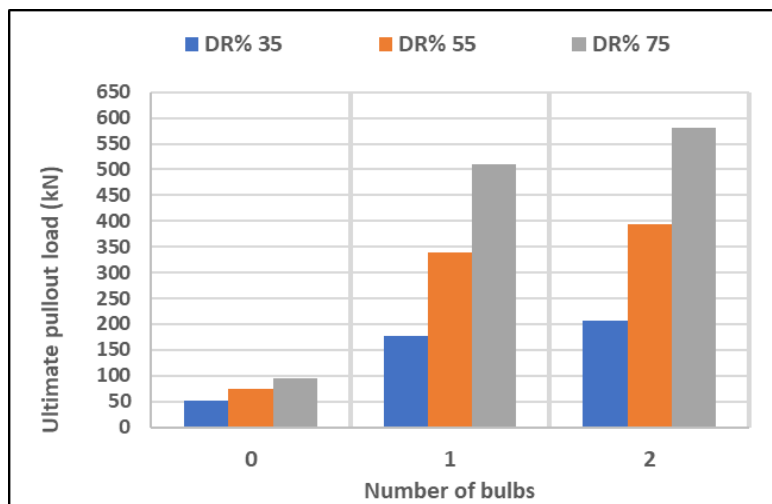
Fig. 10 Effect of the Number of Bulbs on the Ultimate Pullout Load.
