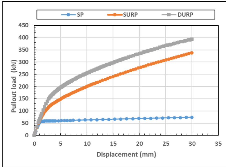
Fig. 7 Load-Displacement Curve in Sandy Soil, Relative Density 55%.
