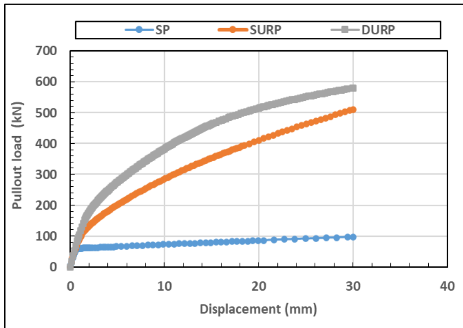
Fig. 8 Load-Displacement Curve in Sandy Soil, Relative Density 75%.
