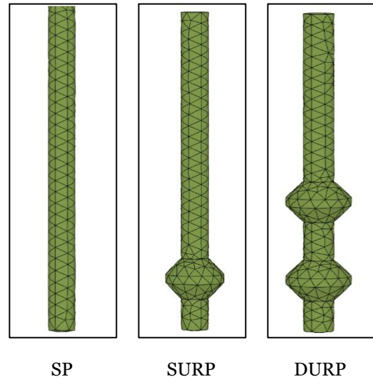
Fig. 4 Modelling Pile System (PLAXIS -3D).
